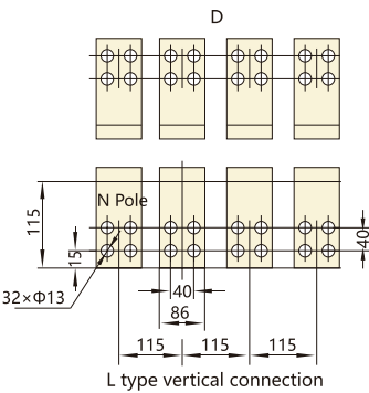
L type vertical connection
