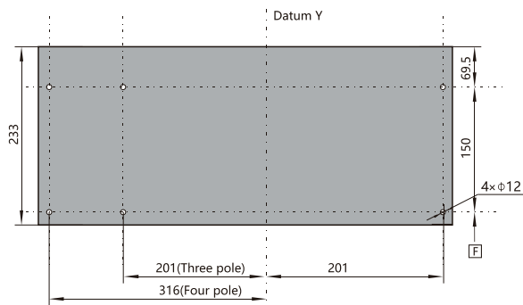
Hole size of the base
