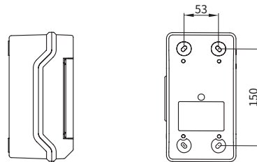
Dimension drawing
