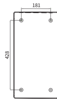
Dimension drawing
