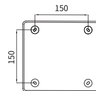
Dimension drawing
