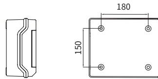
Dimension drawing
