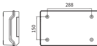
Dimension drawing
